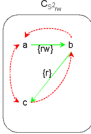
Figure 3. The secure reconfiguration of \mathcal{C}_{S_{rw}^1} as \mathcal{C}_{S_{rw}^2} (Example 4).
