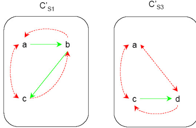
Figure 5. Re-configurations C'_{S1} and C'_{S3} (Example 6).
