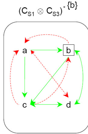
Figure 6. Reconfiguration (\mathcal{C}_{S1} \otimes \mathcal{C}_{S3})^{*\{b\}} (Example 9).
